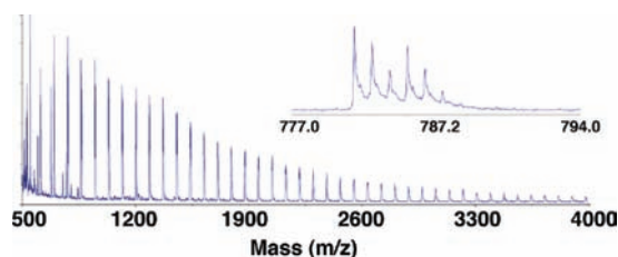
Figure 1. ESI-MS analysis of CPol sample. Conditions: [ 1 ] = 9.8 mM; [ 2 ] = 11.2 mM; [1-Hexene] = 0.47 M; 0.6 mL of toluene- d_8 /0.2 mL of chlorobenzene- d_5 , -40 °C, 3.5 h. Inset shows isotopic resolution.
